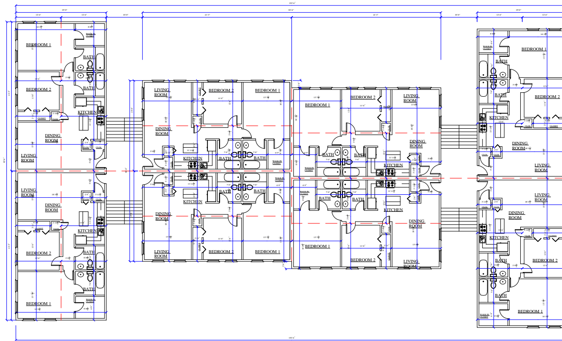
BUILDING #2 FLOOR PLAN SCALE: 1/8" = 1'-0"
